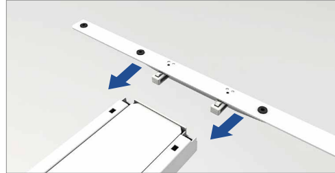
Side Bracket Connection
